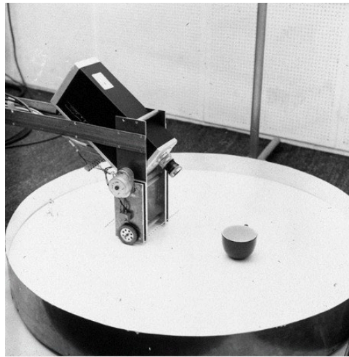
Freddy I identifying a cup. Image © University of Edinburgh
