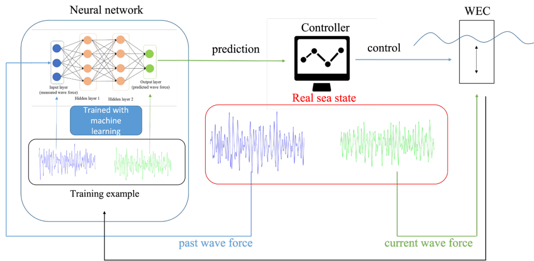
Control block diagram
