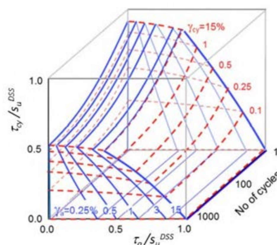
Example 3D cyclic contour diagram for OCR=1 Drammen Clay (reproduced from [1])
