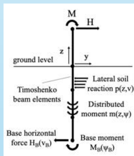
Pisa 1D FE Framework [2]
