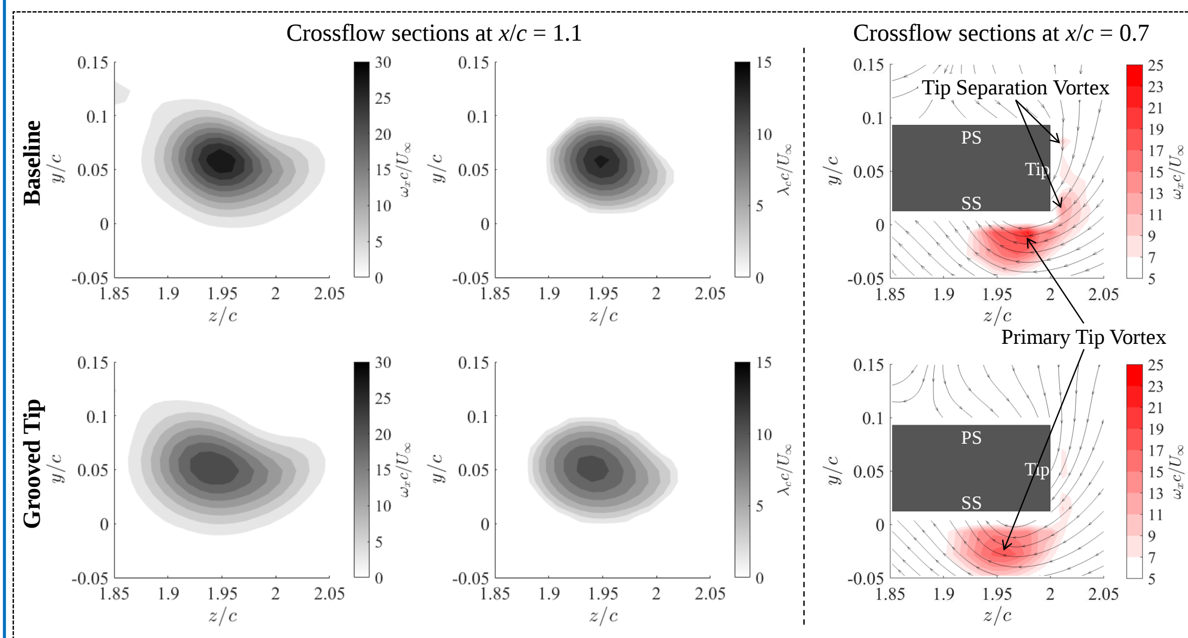
Fig. 4: Crossflow PIV results showing a reduction in vorticity ( \omega_x ) and swirling strength ( \lambda_c ) in the wake with enlarged vortex dimensions (left panel); mitigation of tip separation vortex (right panel).
