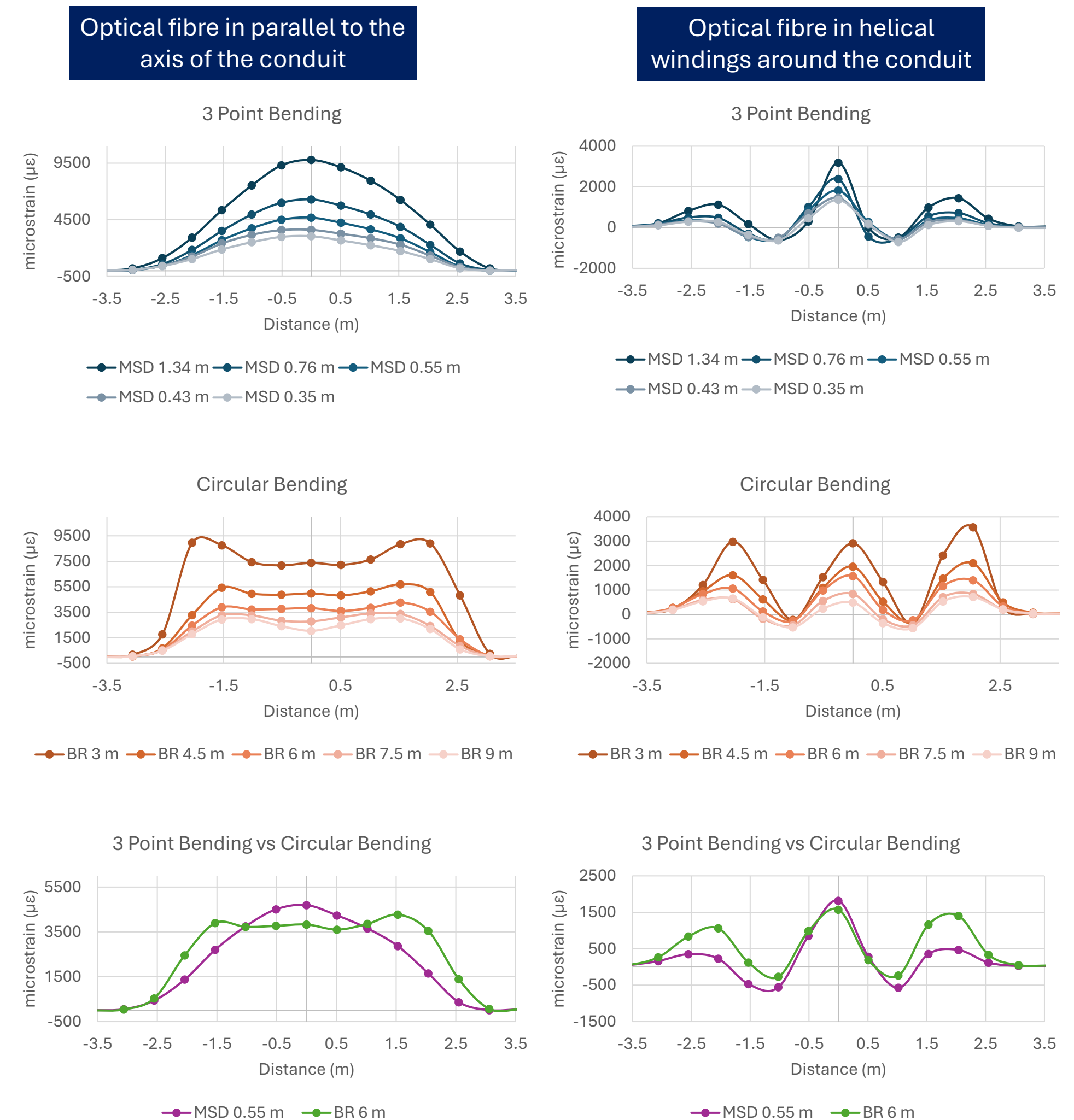
Figure 3: Strain data along the Polybutylene conduit under different magnitudes of the deformation.
