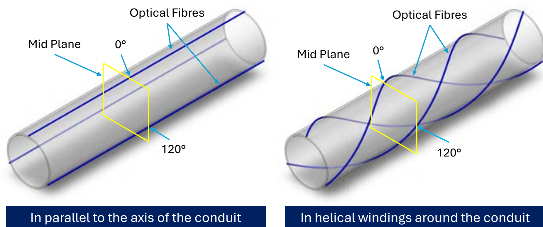
Figure 1: Configurations of the optical fibre attached to the outer surface of the Polybutylene conduit
